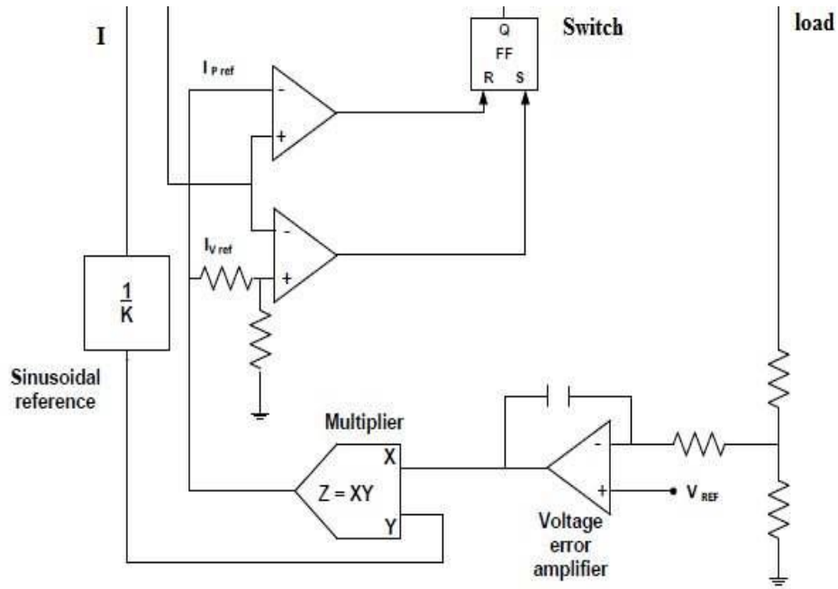
Fig.1. Control circuit for hysteresis control [7]
