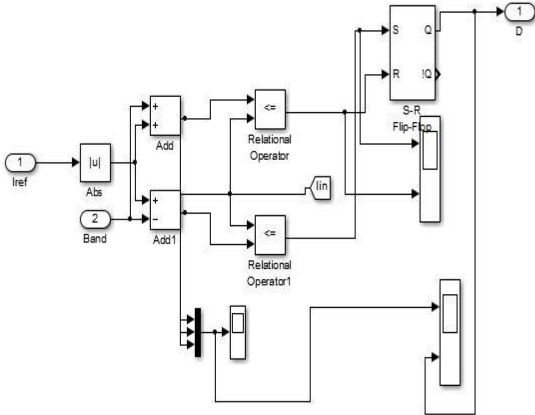
Fig.4. Simulation block diagram of Hysteresis control technique
