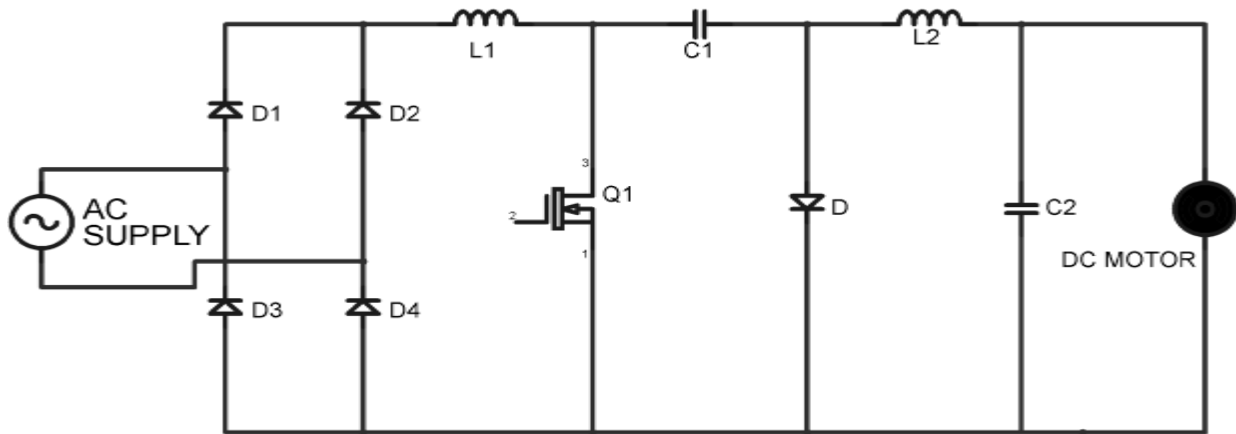
Fig.2. Circuit Diagram of bridge rectifier connected with ĆUK converter
