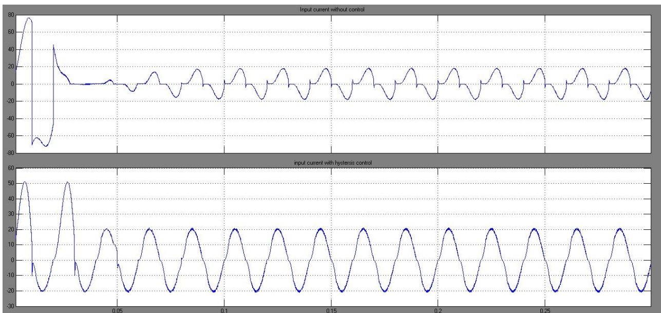
Fig.5. Simulation result of input current without control techniques and with Hysteresis control technique
