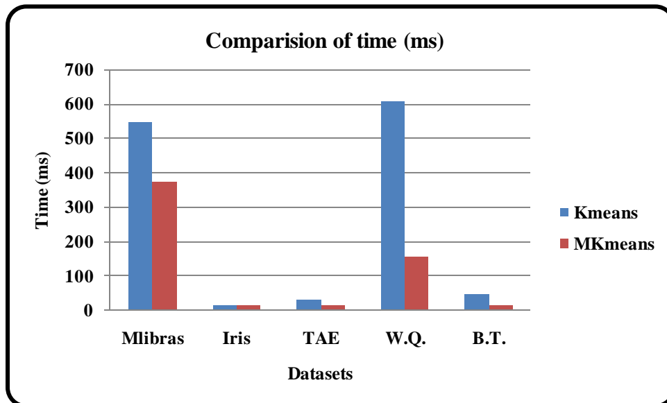
Figure 3: Comparison of Efficiency in Term of time (ms)
