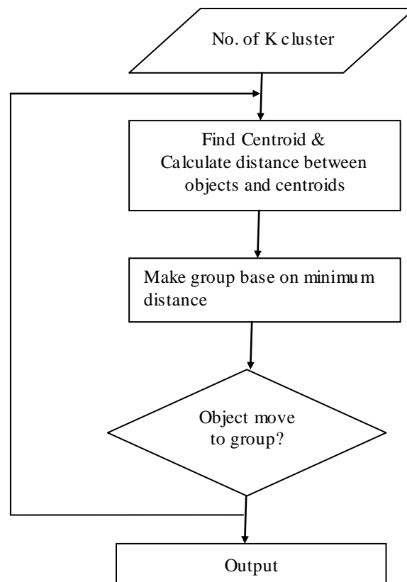
Fig.2 Flowchart of K-mean clustering algorithm
