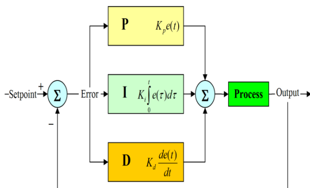
Fig. 2. Schematic of the PID Controller
