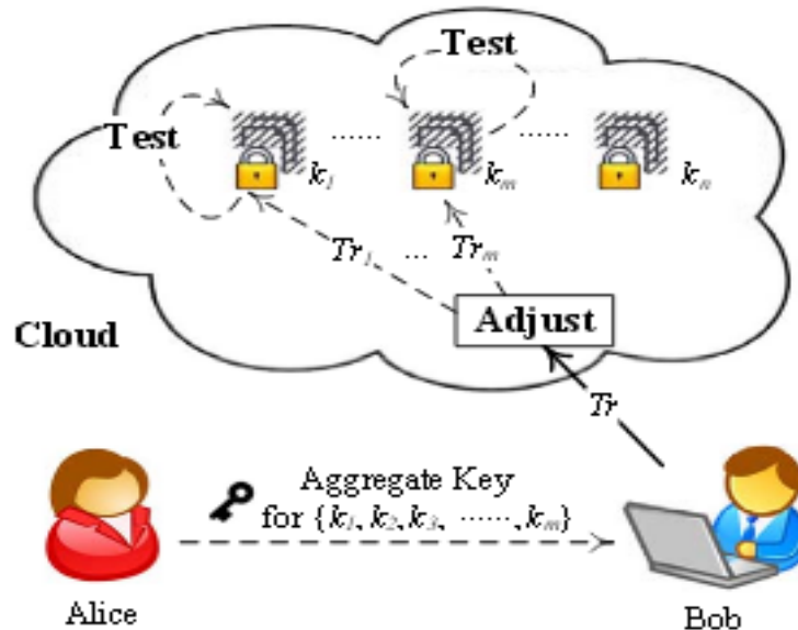
Fig. 2. Framework of key-aggregate searchable encryption.
