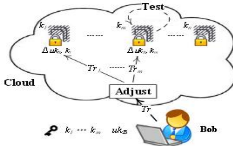
Fig. 1. Multi-Key Searchable Encryption
