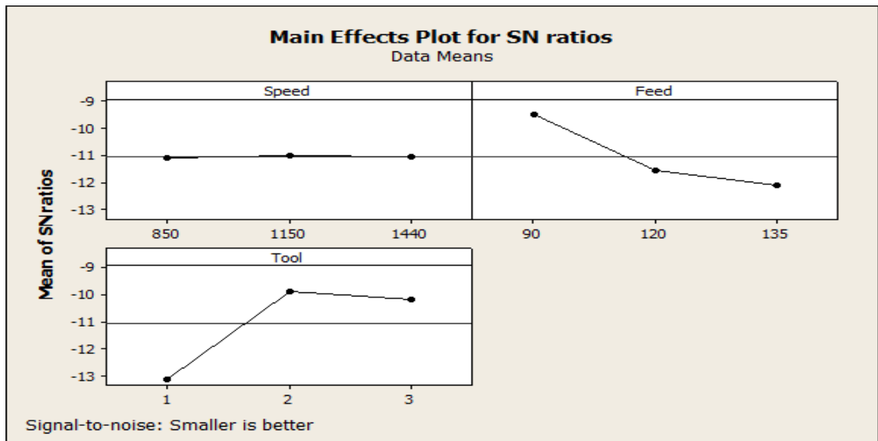
Graph No.1 Main effect plot for S/N ratios of surface roughness
